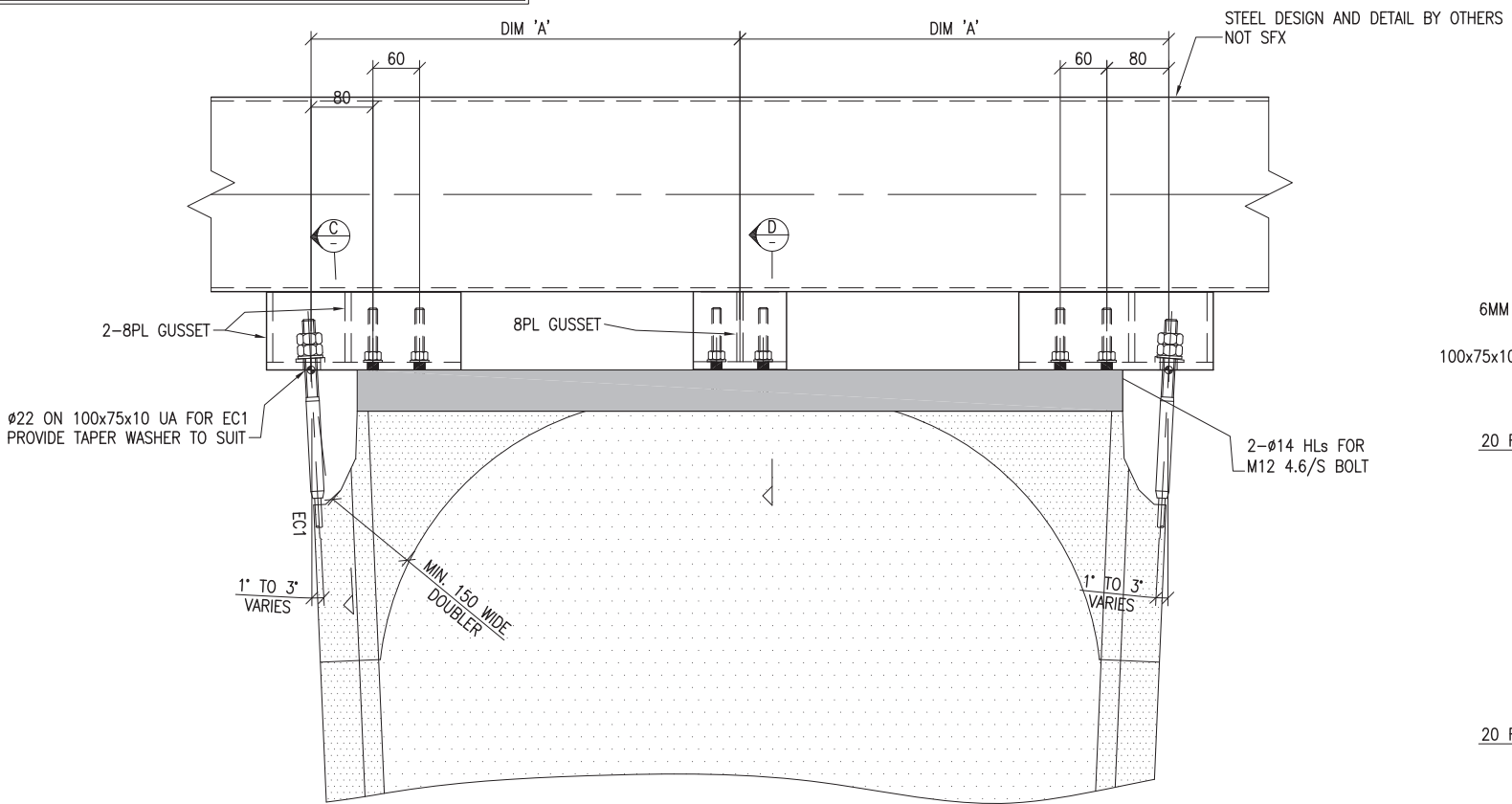
DETAIL 3 1:5
